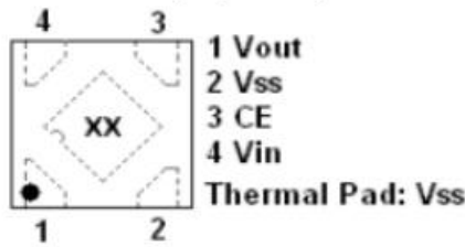
DFN1×1-4(Top view)
