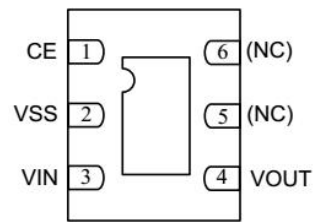
DFN 2*2-6L (Top view)
