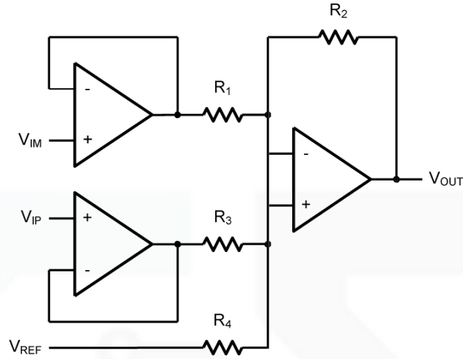
Figure 6. Instrument Amplifier
